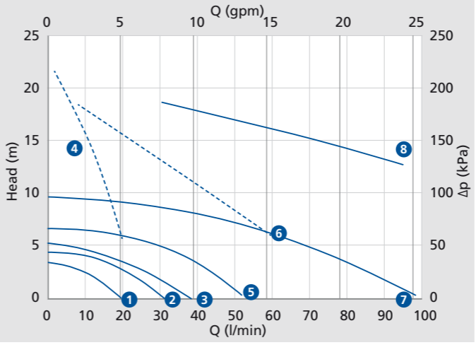
60 Hz water pump curves
