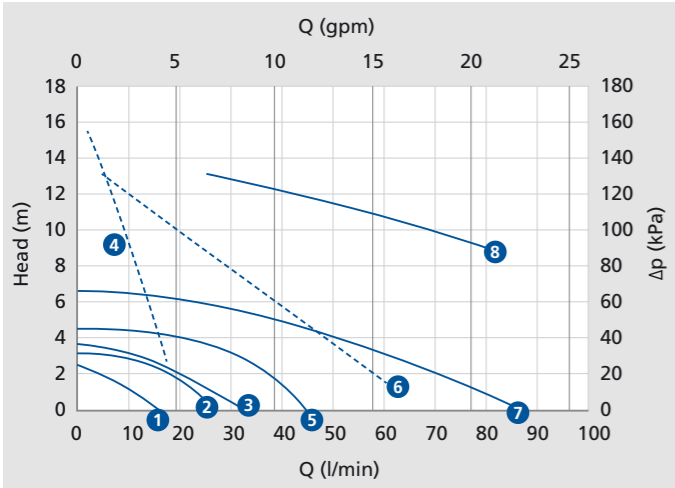
50 Hz water pump curves
